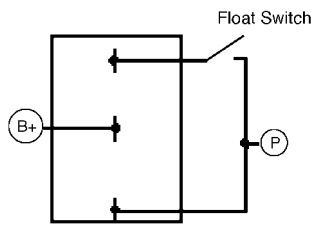
Bilge Pump SPDT ON-OFF-(ON)
