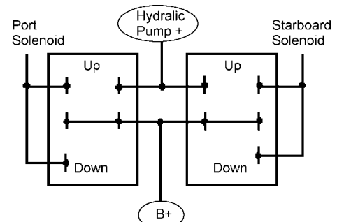
Trimtabs Note: 2 DPDT (ON)-OFF-(ON)
