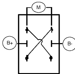
Reversing DPDT
