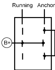
Anchor / Running Lights DPDT ON-OFF-ON
